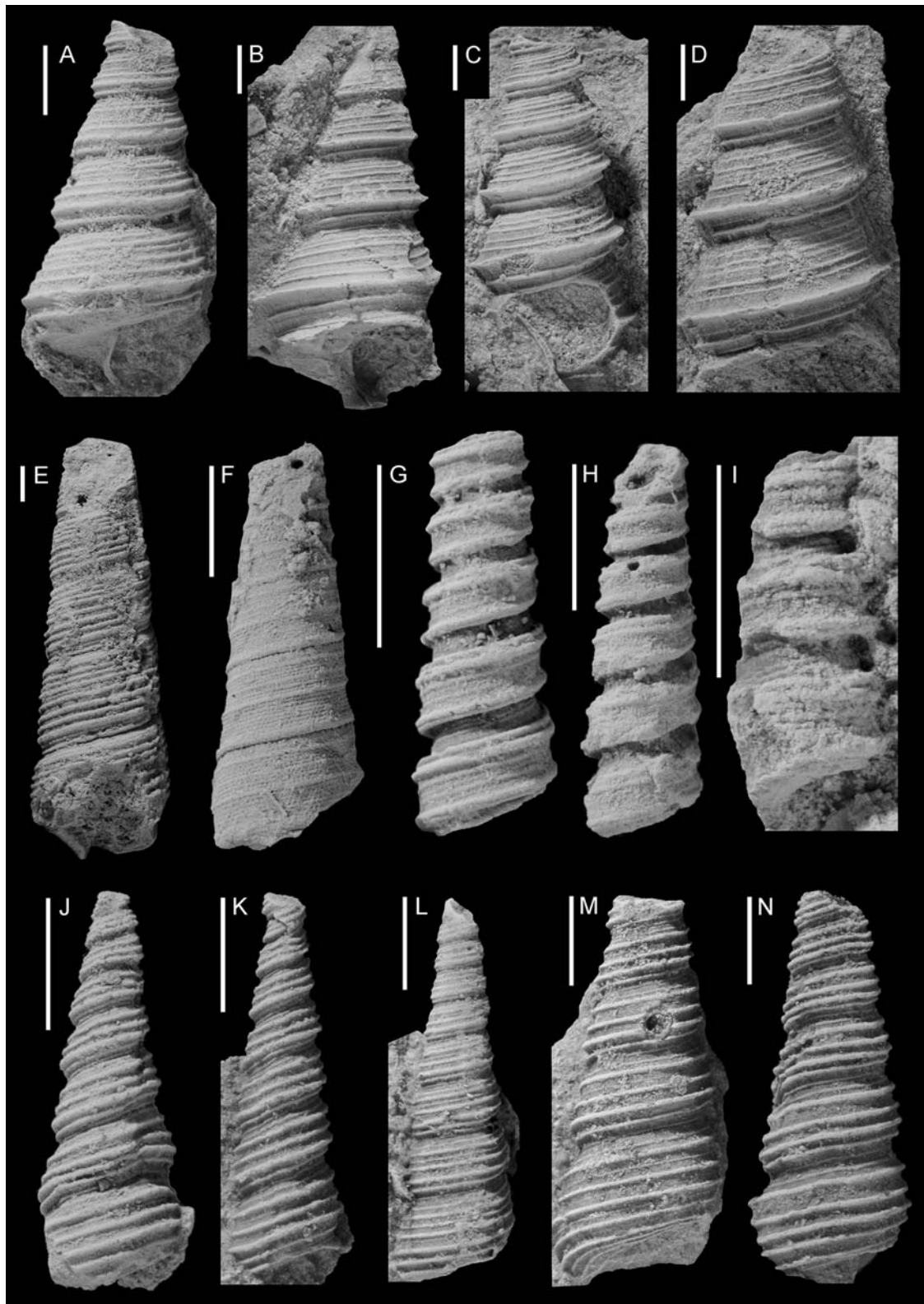
Fig. 3 Turrnellids of the Kutch Basin. a–d Zaria angulata (Sowerby, 1840), NHMW 2008z0256/0002, Khari Nadi River. e Protoma deshayesi (d'Archiac, 1850), NHMW 2008z0256/0001, Khari Nadi River. f Haustator tauropterritus Sacco, 1895, NHMW 2008z0257/
